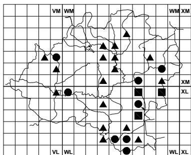
Alyssum granatense
